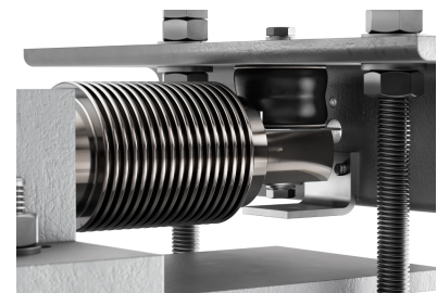
Load cell
